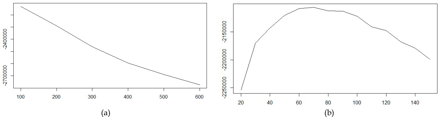
Figure 11-Number of topics (x-axis) and goodness of the model measured with log likelihood measure of the data given the model (y-axis), see [18] for details
