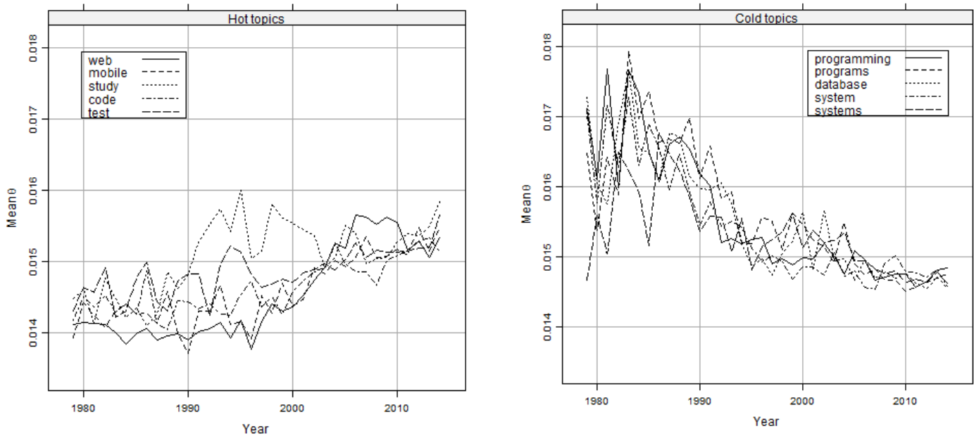
Figure 12- The five hottest and coldest topics
