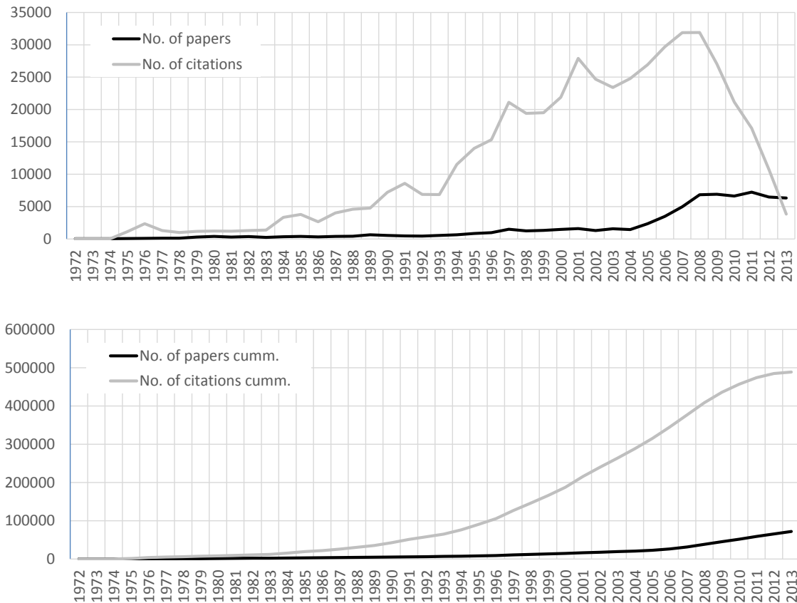
Figure 6- Annual number of papers and citations (top: yearly values, bottom: cumulative trend)
